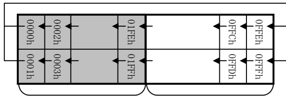
Display area 256dots Hidden area 1792dots
